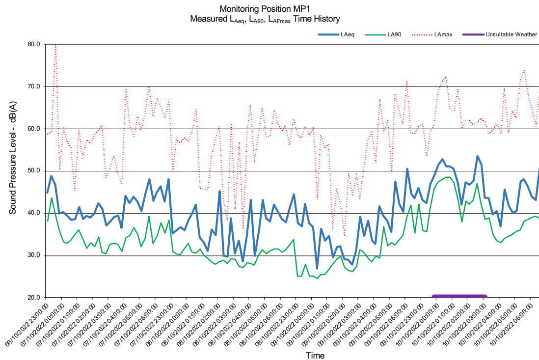
FIGURE 7: MEASURED TIME HISTORY – MP1
