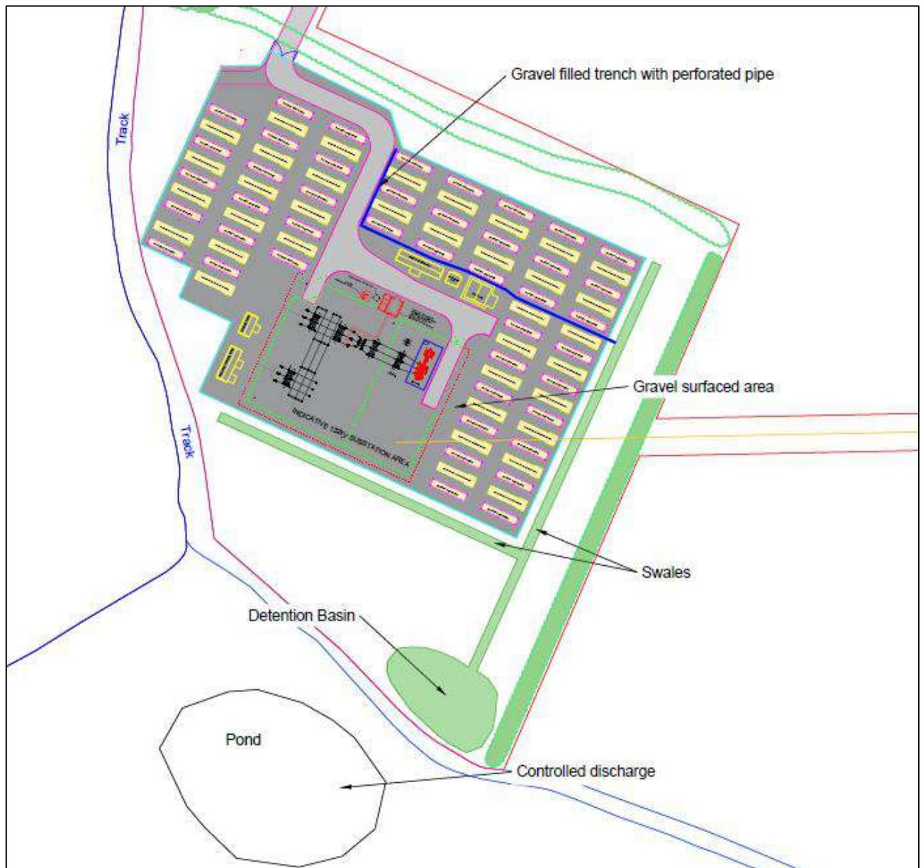
Figure 5.2: Conceptual Drainage Strategy
